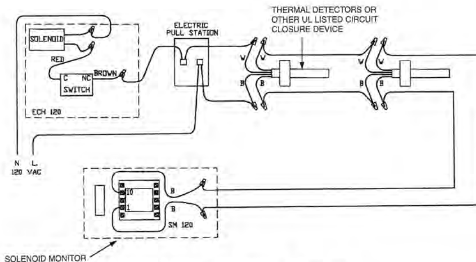
Figure 4-14.1. Wiring Diagram, Solenoid.
