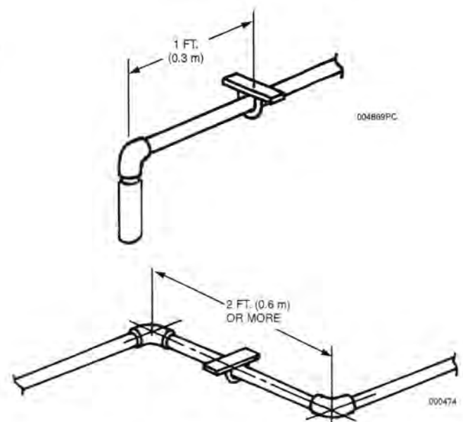
Figure 4-27. Hanger/Support.
