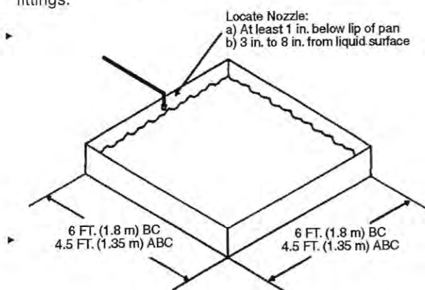
Figure 3-1. N-TS Nozzle Location
