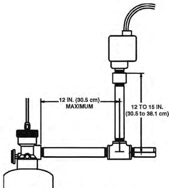
Figure 4-29. Pressure Switch Installation.
