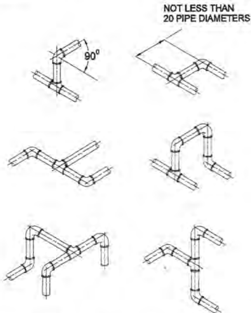
Figure 4-25. Acceptable Piping Methods.
