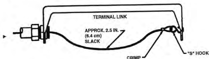
Figure 4-9. Terminal Bracket Connection.
