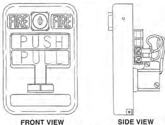
Figure 2-13a. Model RPS-E2 Remote Electric Pull Station.
