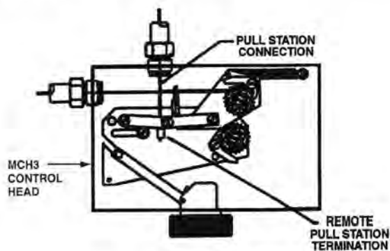
Figure 4-17. Model RPS-M Remote Pull Station Termination.
