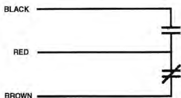
Figure 4-23. Wiring Diagram For Model MS-SPDT Micro Switch.
