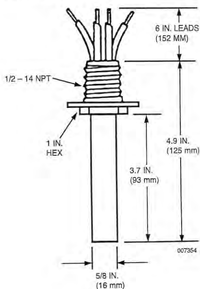
Figure 2-12a. Thermal Detector.
