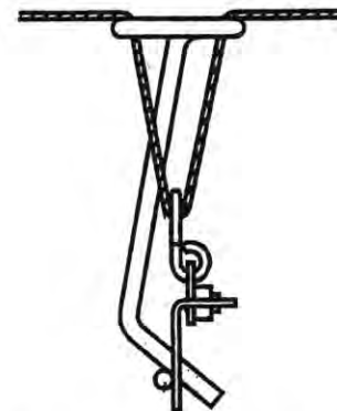
Figure 4-11. Fusible Link/Hanger Connection.
