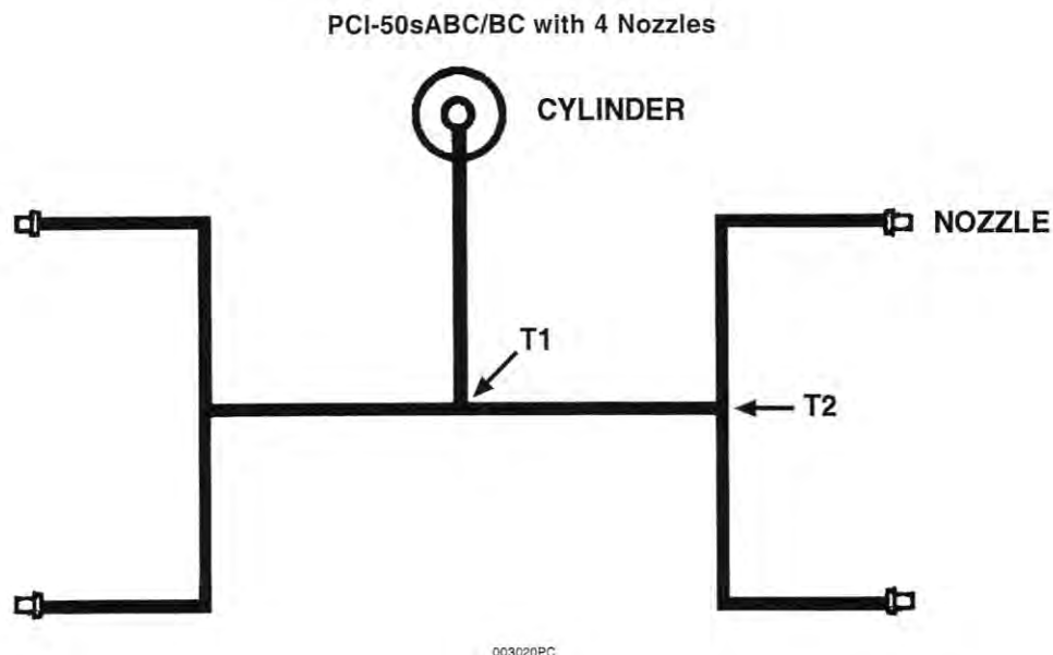
Tankside Piping Limits PCI-50sABC
