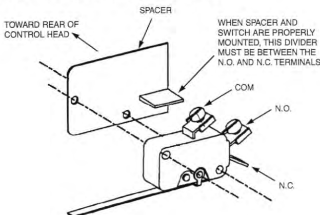
Figure 2-20b. Alarm Initiating Switch.
