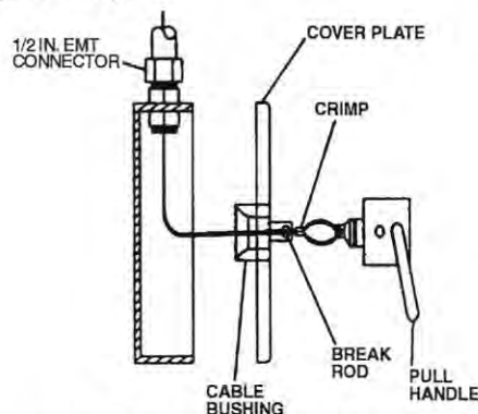
Figure 4-16. Model RPS-M Remote Pull Station Installation.
