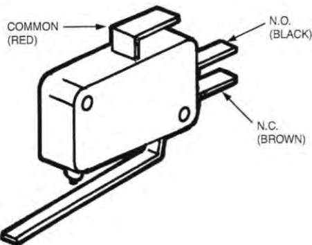
Figure 2-20a. Model MS-SPDT Micro Switch.
