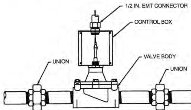
Figure 4-18. Gas Valve Installation.
