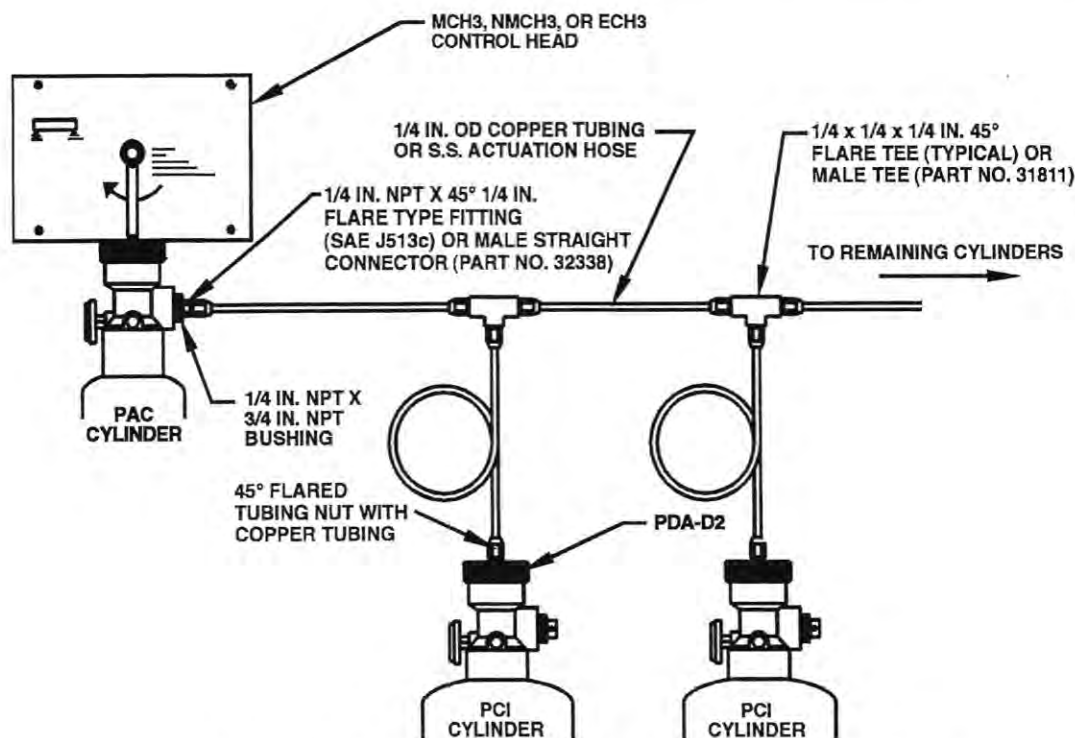
Figure 4-5. Multiple Cylinder Actuation Using Model PAC-10 or PAC-200
