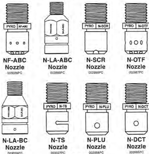
Figure 2-3. Nozzles.
