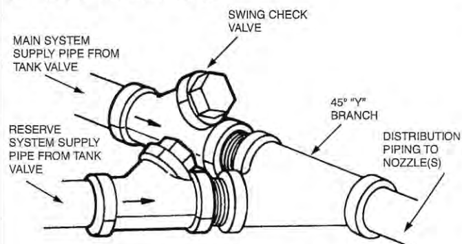
Figure 4-28. Main/Reserve System.
