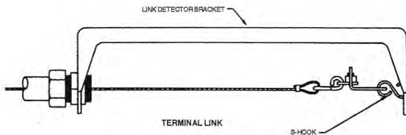
Figure 4-6. Terminal Link Installation.
