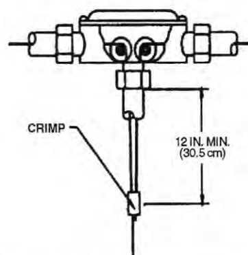
Figure 4-20. Tee Pulley Installation.
