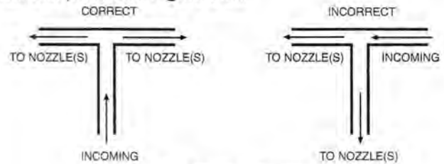
Figure 4-26. Tee Positioning
