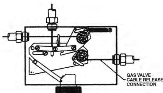
Figure 4-19. Gas Valve Line Termination.
